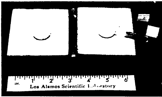
Fig. 5. Thermocouple installation for a 25-mm sphere.
