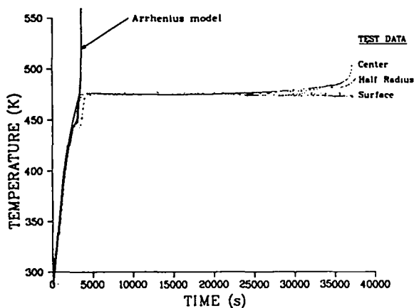
Fig. 10. Comparing the test data with the analytical model for PBX 9501 shows that an induction process is impeding the reaction.
