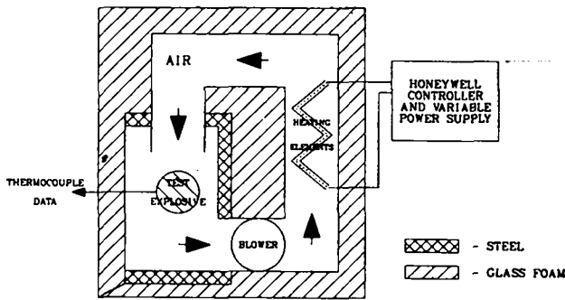
Fig. 2. Critical-temperature test chamber for unconfined spheres up to 80 mm in diameter.
